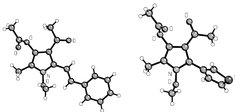
Figure 6. Molecular structures of 16d (left) and 16e (right), as obtained by X-ray crystallography.
