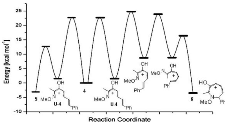
Figure 3. Energy profiles for the cyclization of cation 4 to form either five-membered heterocyclic system 5 or seven-membered ring system 6 [SCS-MP2/6-31G(d)//RHF/6-31G(d)].
