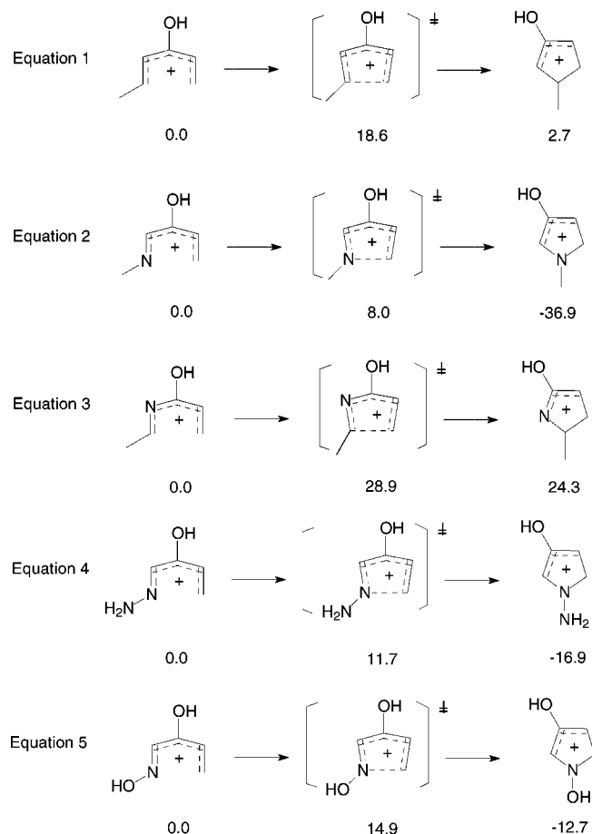
Figure 1. Cyclization reactions of 3-hydroxypentadienyl and various aza-3-hydroxypentadienyl systems. Relative energies [kcal/mol] with respect to the starting material are given for the transition states and the cyclic products (G3 level of theory).
