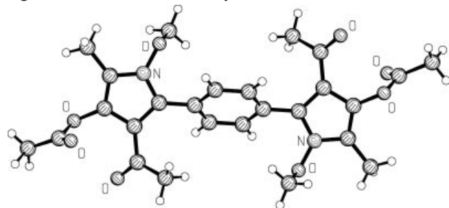
Figure 7. Molecular structure of compound 17a , as obtained by X-ray diffraction.
