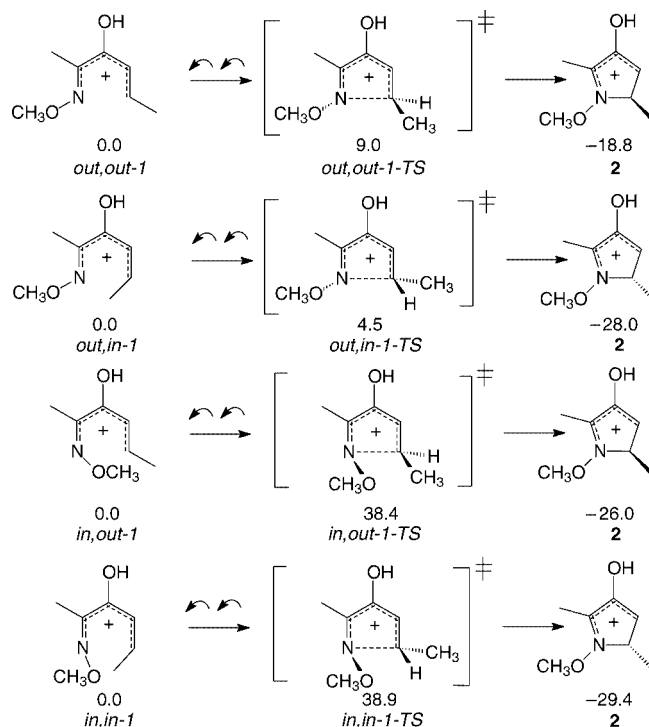
Figure 2. Four different modes for the cyclization reaction of 3-hydroxy-1-methoxy-1-azapentadienylium ion 1 to give 2 . Relative energies were calculated at the SCS-MP2/6-31G(d)//RHF/6-31G(d) level of theory and are given in kcal/mol.
