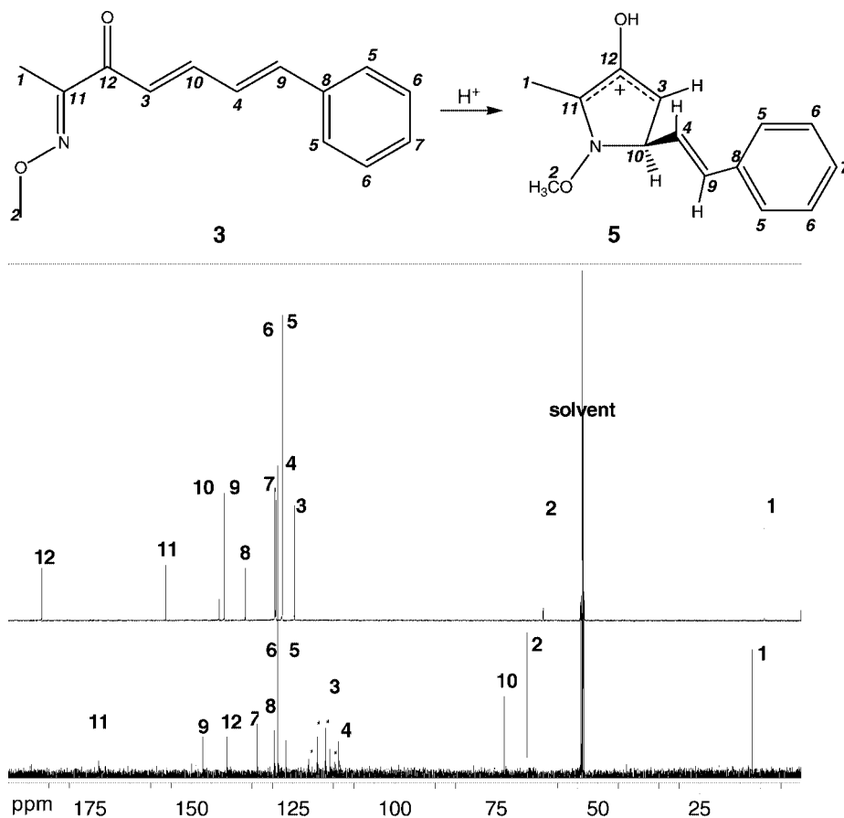
Figure 5. ^{13}\text{C} NMR spectra for the protonation of 3 with numbering scheme for the carbon atoms. Upper spectrum: compound 3 before addition of trifluoromethanesulfonic acid (room temperature); lower spectrum: after addition of the acid to form 5 ( \text{CD}_2\text{Cl}_2 , -60\text{ }^{\circ}\text{C} , 100 MHz). The signals from \text{CF}_3 are marked with asterisks.
