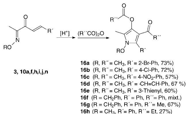
Scheme 9.
