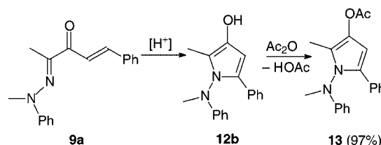
Scheme 6.
